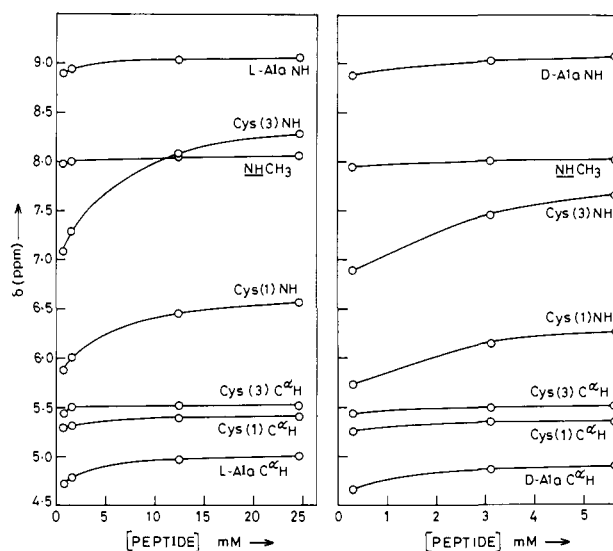
Figure 2. Concentration dependence of NH and C ^\alpha H chemical shifts in CDCl 3 for peptides 1 (left) and 2 (right).
