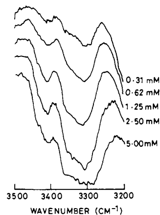
Figure 6. Partial IR spectra (NH stretching region) of 2 as a function of concentration in \text{CHCl}_3 solution.
