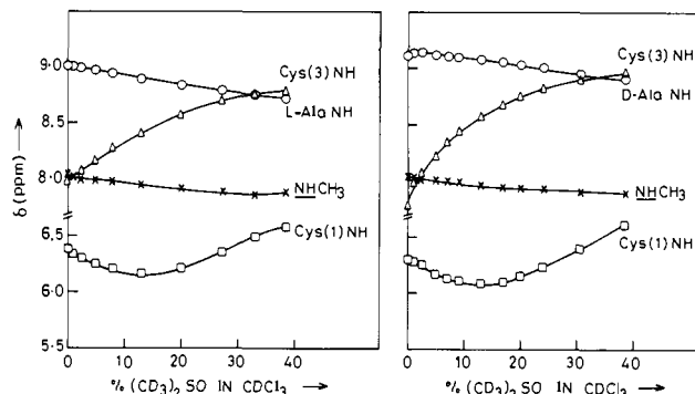
Figure 5. Solvent dependence of NH chemical shifts in \text{CDCl}_3 - (\text{CD}_3)_2\text{SO} mixtures as a function of solvent composition for (left) 1 and (right) 2 .
