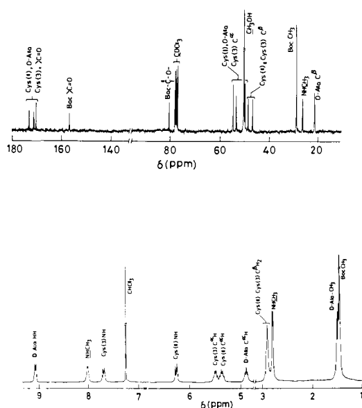
Figure 1. ^1\text{H} (270 MHz) (bottom) and ^{13}\text{C} (67.89 MHz) (top) NMR spectra of peptide 2 in CDCl 3 .
