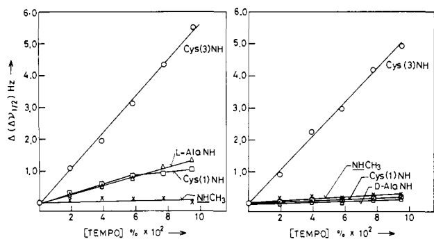
Figure 3. Line broadening of peptide NH resonances as a function of TEMPO concentration in \text{CDCl}_3 for 1 (left) and 2 (right).
