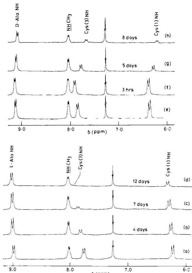
Figure 4. Hydrogen-deuterium exchange of NH resonances in a \text{CDCl}_3 - \text{D}_2\text{O} mixture: (a-d) 1 , (e-h) 2 . Time intervals after \text{D}_2\text{O} addition are indicated on the traces.
